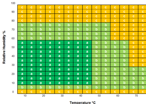
Figure 1: Humidity Sensor Operating Range
